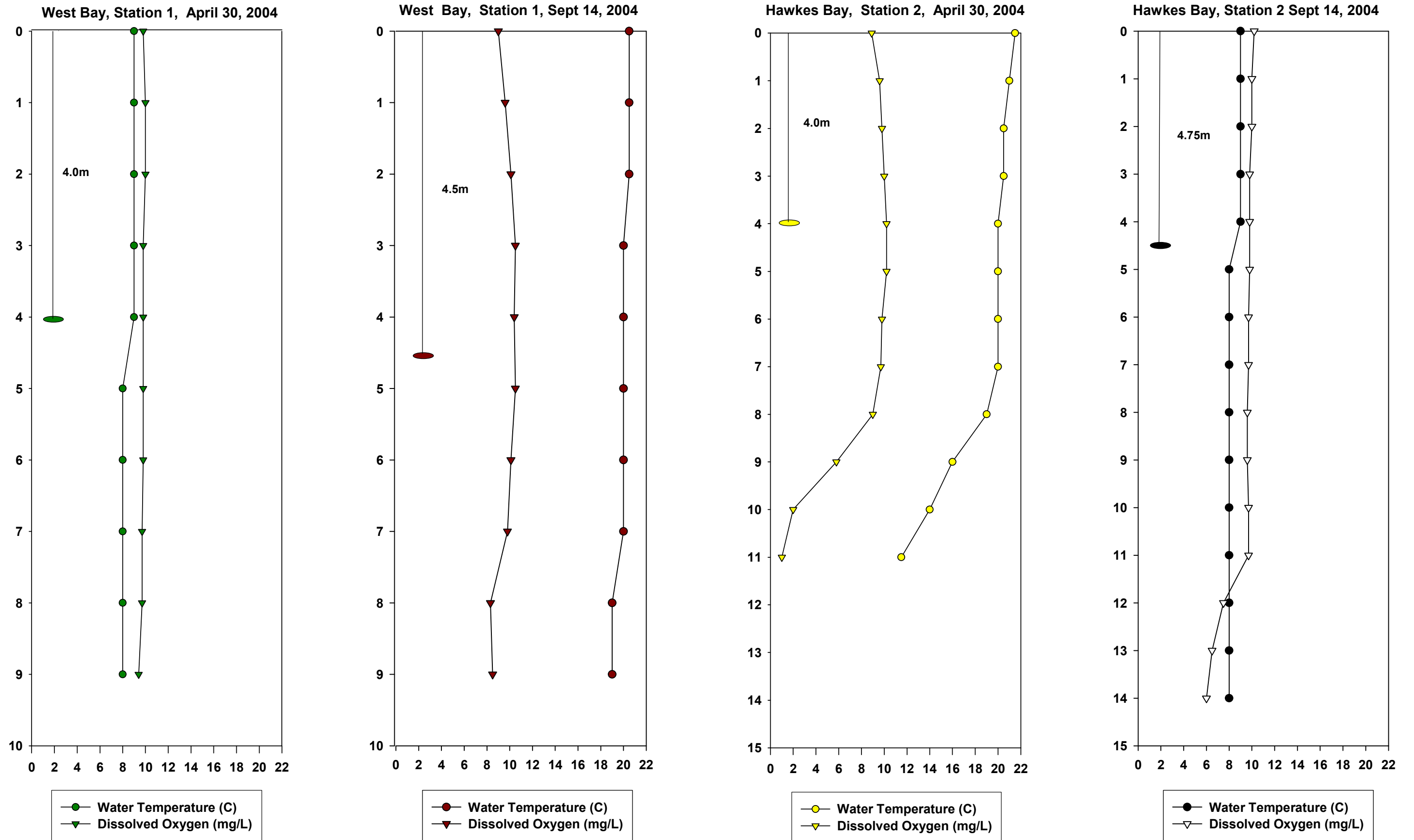
Figure 2. Temperature and dissolved oxygen profiles in Chandos Lake at Stations 1 and 2 on April 30, 2004 and on Sept 14, 2004. Secchi disc values are also shown in top left. Data were collected by Michalski Nielsen Associates Limited.
