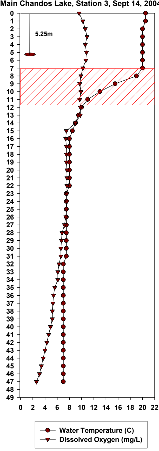
Figure 4. Temperature and dissolved oxygen profiles in Chandos Lake at Stations 3 and 4 on April 30 and September 14, 2004. Secchi disc values are also shown in top left. Locations of metalimnia are shown in hatched areas. Data were collected by Michalski Nielsen Associates Limited.
